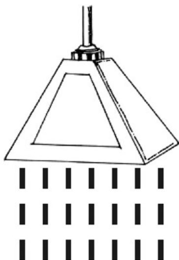
A hood for an even flat fan nozzle showing spray direction
