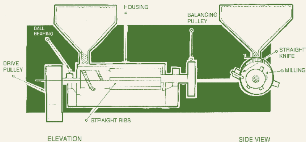
Plate 1.13 Engleberg grain dehuller used for maize, rice or sorghum
