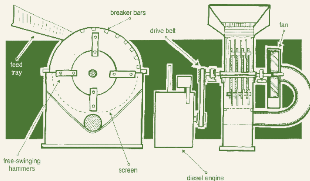
Plate 1.12 Hammer mill
