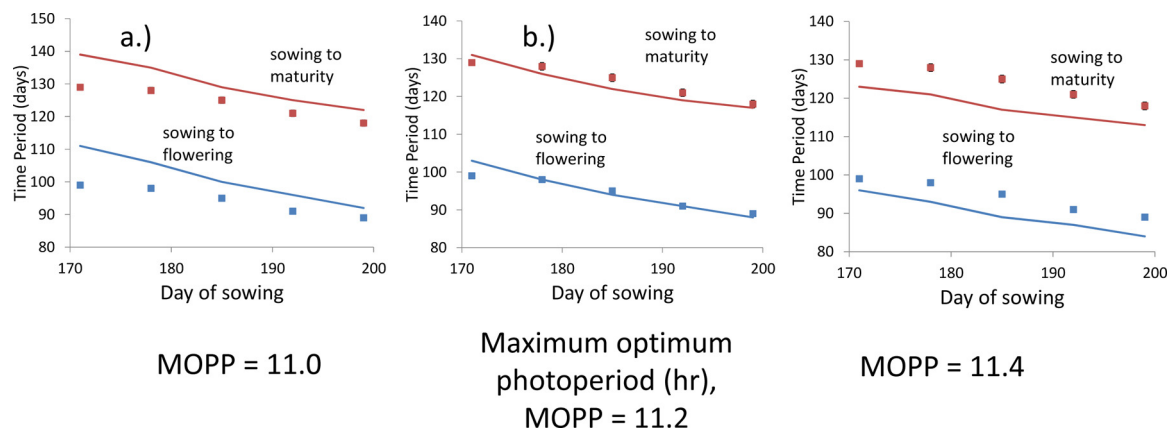
Fig. 7. Sensitivity of APSIM-Oryza varietal optimum photoperiod parameter (MOPP) in simulation of rice sowing date trial, Chuadanga, Bangladesh (Dataset # 13; Rashid et al., 2009); a.) MOPP = 11 h, b.) MOPP = 11.2 h, and c.) MOPP = 11.4 h.
