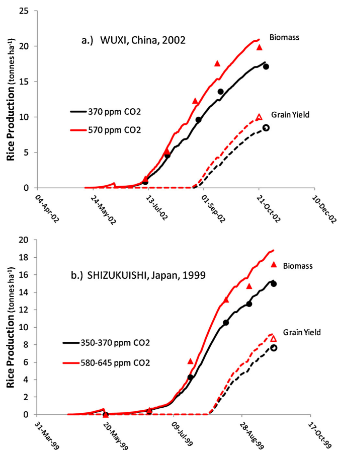
Fig. 17. APSIM-Oryza simulated versus observed rice production ( \text{Mg ha}^{-1} ) for both FACE and ambient \text{CO}_2 treatments: (a.) Yang et al., 2006, 2008 (dataset # 25); (b.) Kim et al., 2003 (dataset # 24). Comparison for medium N treatments shown. No replicate variability information (error bars) available.
