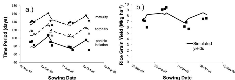
Fig. 8. Simulated and observed data for a rice sowing date trial over two years, Andhra Pradesh, India (Rao and Reddy, 1998; dataset #41). Graphs show a.) crop phenology; and b.) crop production, for a non-photoperiod-sensitive rice cultivar (BPT-5024), in contrast to Fig. 5 (photoperiod sensitive).
