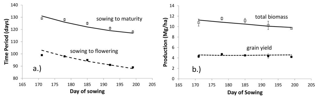
Fig. 5. Simulated and observed data for sowing date trial of T.Aman rice, Chuadanga, Bangladesh (Dataset #13; Rashid et al., 2009). Graphs show a.) crop phenology; and b.) crop production, for a strongly photoperiod-sensitive rice cultivar (BR11). Simulated data represented by lines; observed data by points with error-bars representing the variability across replicates (one standard deviation either side of the mean).
