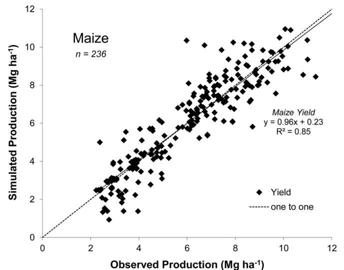
Fig. 3. Comparison between observed and simulated grain yields (Mg ha -1 ) for maize.
