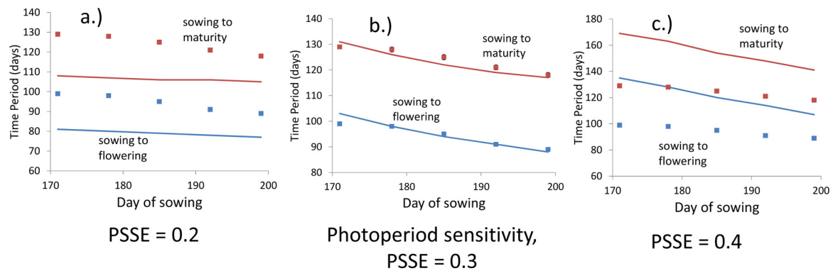
Fig. 6. Sensitivity of APSIM-Oryza varietal photoperiod sensitivity parameter (PSSE) in simulation of rice sowing date trial, Chuadanga, Bangladesh (Dataset # 13; Rashid et al., 2009); a.) PSSE = 0.2, b.) PSSE = 0.3, and c.) PSSE = 0.4.
