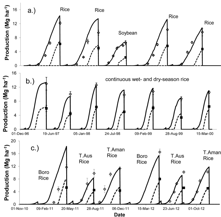
Fig. 10. Three example multi-crop sequence experiments in rice-based systems, simulated using APSIM – each conducted with continuous simulation of multiple crops and fallows without resetting soil variables (water and nutrients) between crops. Treatments illustrated: – (a) Suriadi et al., 2009 ( N = 150 \text{ kg ha}^{-1} , continuous flooding, Lombok, Indonesia; dataset # 2); (b) Boucher 2001 (late tillage, minus straw, plus N, at IRRRI Los Baños, Philippines; dataset # 4); (c) Gaydon et al., 2013 (T2–boro–T.Aus–T.Aman rotation at Gazipur, Bangladesh; dataset # 7). The continuous lines represent model output (solid– above-ground biomass; broken – grain yield); the discrete points with error bars are the observed values (error bars representing one standard deviation either side of the mean). The open symbols above-ground biomass, the closed are grain yield.
