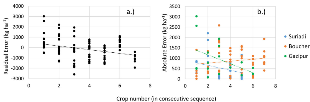
Fig. 11. The dynamics of (a) combined residual error, and (b) individual dataset absolute error in grain yield ( \text{kg ha}^{-1} ) with advancing crop number in three APSIM simulated crop sequence experiments, each conducted with continuous simulation of multiple crops and fallows without resetting soil variables (water and nutrients) between crops. (a) Suriadi et al., 2009 (dataset # 2); (b) Boucher 2001 (dataset # 4); (c) Gazipur (Gaydon et al., 2013 (dataset # 7)). The data points above were generated using average error across all treatments and replications in each dataset.
