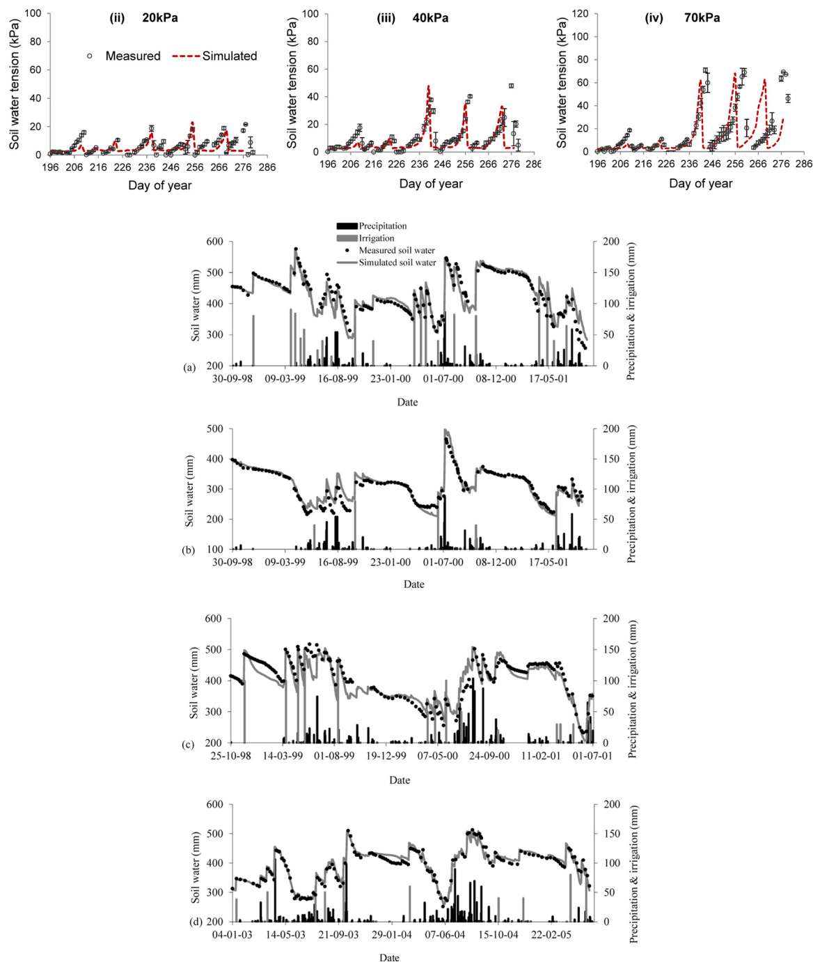
Fig. 12. (a) Comparison between observed and simulated soil moisture (kPa – 0–15 cms soil depth) for different water-stress treatments in rice irrigation, Punjab, India – (i) CS – control, continuously submerged/flooded (not shown); (ii) AWD, re-flooded at soil suction of 20 kPa; (iii) AWD, 40 kPa; and (iv) AWD, 70 kPa, for the experiments of Sudhir-Yadav et al. (2011a,b) (Dataset #5). (b) Comparison between observed and simulated soil moisture (mm – 0–160 cms soil depth) for irrigation treatments in wheat irrigation at Luancheng, China, 1998–2001–(i) irrigation at critical growth stages; (ii) irrigation at sowing only; (iii) at Yucheng (d) AWD, 70 kPa, for the experiments of Chen et al. (2010b) (Dataset #31). (c) Comparison of simulated and observed volumetric soil water content ( \text{cm}^3 \text{cm}^{-3} ) under wheat in the soil profile (0–90 cm soil depth) with and without mulching during the 2007–08 wheat season in irrigation treatment I2, Punjab, India (Balwinder-Singh et al., 2011; dataset # 38).
