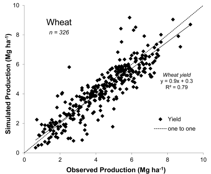
Fig. 2. Comparison between observed and simulated grain yields (Mg ha -1 ) for wheat.
