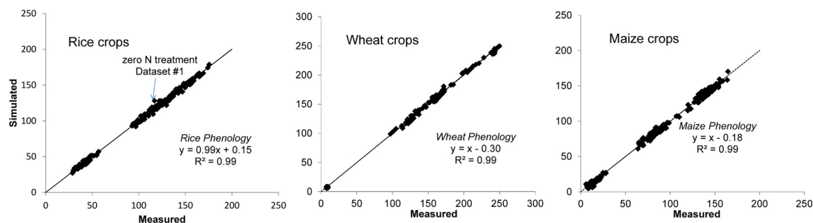
Fig. 9. Comparison between observed and simulated phenology dates (days after sowing) for rice, wheat and maize (validation data-points only shown). Stages shown include panicle initiation (PI), anthesis (A) and physiological maturity (PM) for rice; and emergence (E), A and PM for wheat and maize.
