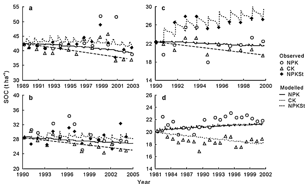
Fig. 16. Comparison between observed and simulated soil organic carbon ( \text{t ha}^{-1} ) for the experiments of Wang et al., 2014. (dataset # 27). A mixture of wheat and wheat-maize cropping systems were examined over four (4) Chinese locations, over a period of 20+ years with a range of fertiliser and stubble treatments. NPK = application of compound inorganic fertilizers; NPKSt = application of inorganic fertilizers and stubble retention; CK = control. Symbols show the observed values and lines show the simulated values.
