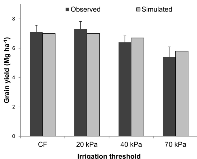
Fig. 14. Comparison between observed and simulated above-ground rice grain yield ( \text{Mg ha}^{-1} ) for different water-stress treatments in rice irrigation – (i) CS – control, continuously submerged/flooded; (ii) AWD, re-flooded at soil suction of 20 kPa; (iii) AWD, 40 kPa; and (iv) AWD, 70 kPa, for the experiments of Sudhir-Yadav et al. (2011a,b) (dataset # 5).
