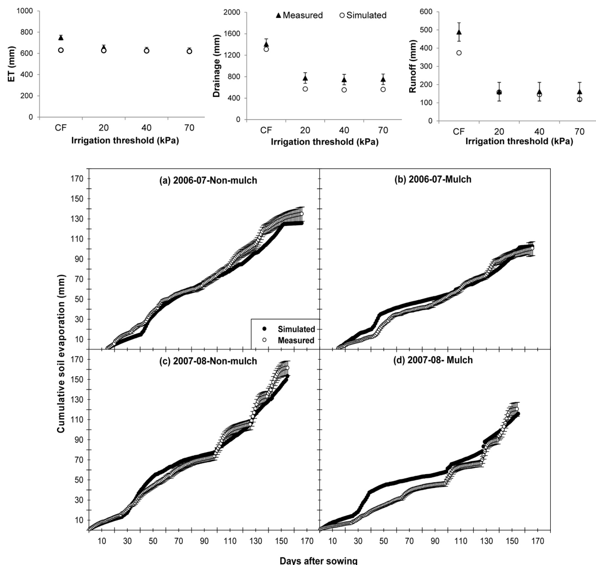
Fig. 13. (a) Comparison between observed and simulated water balance components (mm) as a function of different water-stress treatments in rice irrigation – (i) CF – control, continuously submerged/flooded; (ii) AWD, re-flooded at soil suction of 20 kPa; (iii) AWD, 40 kPa; and (iv) AWD, 70 kPa, for the experiments of Sudhir-Yadav et al. (2011a,b) (dataset # 5). (b) Simulated (filled symbols) and observed (hollow symbols) cumulative soil evaporation under mulch and non-mulch in 2006–07 (a. and b.) and 2007–08 (c. and d.) for irrigated wheat crops, Punjab, India (Balwinder-Singh et al., 2011; dataset # 38).
