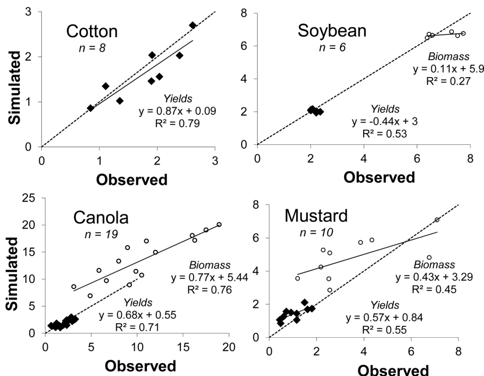
Fig. 4. Comparison between observed and simulated grain yields and above-ground biomass (Mg ha -1 ) for cotton, soybean, mustard, and canola.
