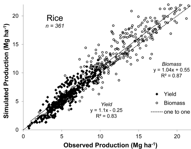
Fig. 1. Comparison between observed and simulated grain yields and above-ground biomass (Mg ha -1 ) for rice.
